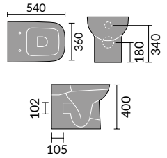
Bordeaux Flush to Wall Toilet
