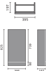
AVIOR COUNTERTOP TAP POSITION GUIDE
