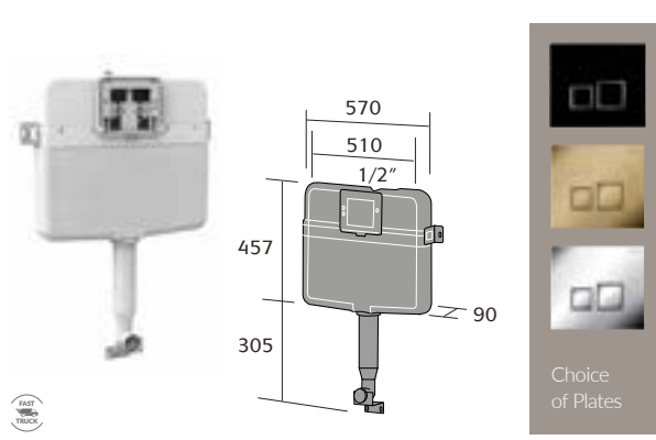
Back to Wall Slim Concealed Cistern @POCCA
