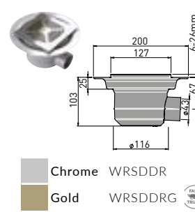
Smart Deck Drain Grid
