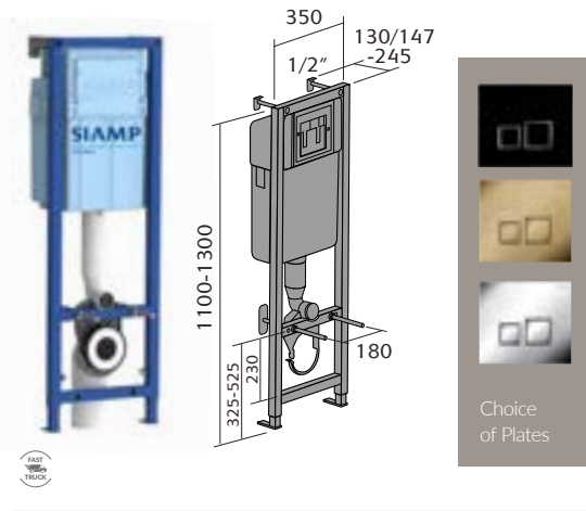
Wall Hung Easy Fit Frame and Connector Kit @POWHAF
