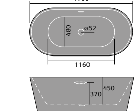
Oval Freestanding Bath 1700x800mm
