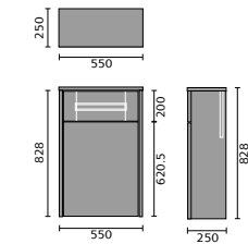
Classic WC Unit
