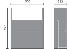
Vanity 500mm
