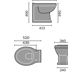
Classic Open Backed Toilet
