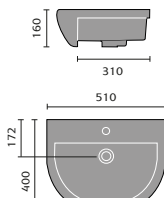
Spacesaver Square Semi Recessed Basin
