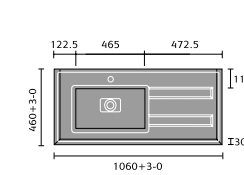
Delphina 1000 Vanity LH Basin
