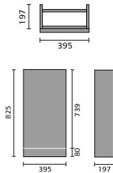
Avior 40cm Floor Standing Compact
