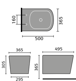
Imperia Wall Hanging Toilet
