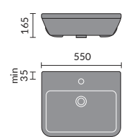
Spacesaver Soft Round Semi Recessed Basin
