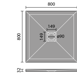
800mm Square
