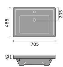
Classic 700 Basin
