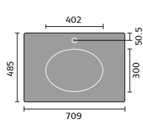
Classic 700 Countertop
