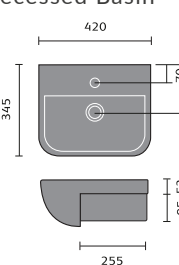
Spacesaver Soft Round Semi Recessed Basin
