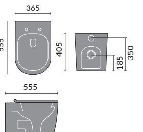
Trivento Back To Wall Toilet
