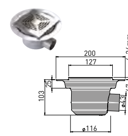
Smart Deck Drain WRSDDR
