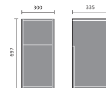
Drawer 300mm
