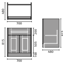
Classic 700 Vanity Floor Standing
