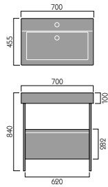
Carina Tall Cabinet
