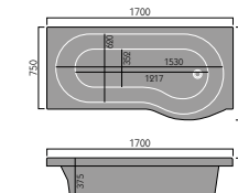
Round Showerbath 1700x850mm LH or RH (RH shown)
