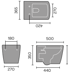
Ceriana Back To Wall Toilet
