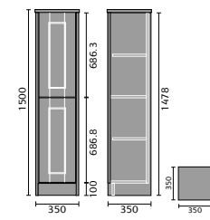
Classic WC Unit
