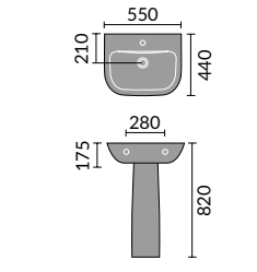
Bordeaux 55cm Basin 1th Semi Pedestal
