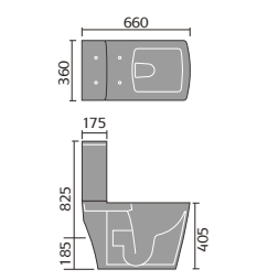
Ceriana Open Backed Toilet
