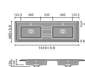
Delphina 1400 Vanity Basin
