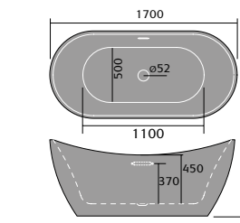
Oval Freestanding Bath 1700x800mm
