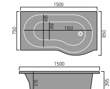
Round Showerbath 1500x850mm LH or RH (RH shown)
