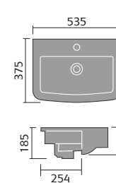
Florence 51cm Semi Recessed Basin
