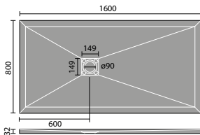
1600x800mm Rectangular
