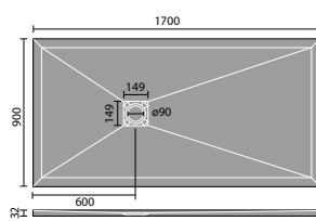
1700x900mm Rectangular
