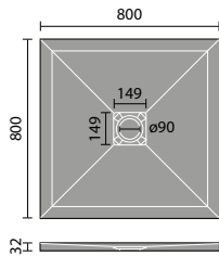
800mm Square
