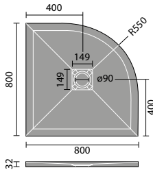
800mm Quad
