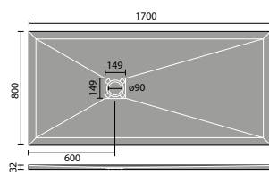
1700x800mm Rectangular
