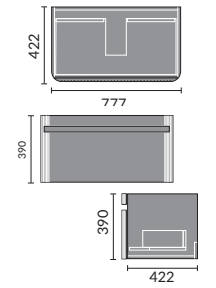
Pavo 800 Vanity
