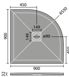
900mm Quad
