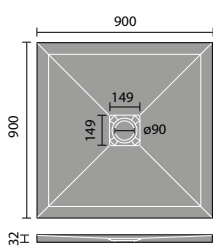
900mm Square
