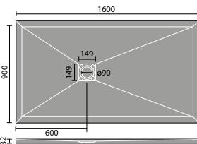
1600x900mm Rectangular
