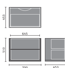
Delphina 700 Vanity
