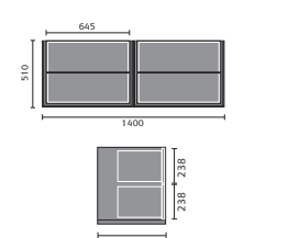
Delphina 1400 Vanity
