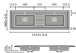
Delphina 1400 Vanity
