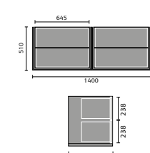
Delphina 1400 Vanity
