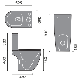
Trivento Open Backed Toilet
