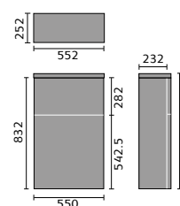
Carina WC Unit
