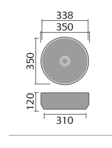
Round Countertop Basin
