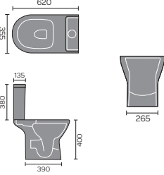
Provence Open Backed Toilet
