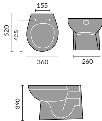
Rimini Back To Wall Toilet
