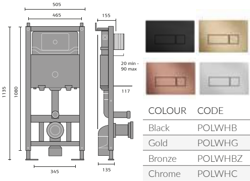
Luxury Wall Hanging WC Frame and Cistern @POLWHF
