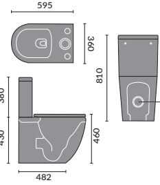
Trivento Flush To Wall Toilet
