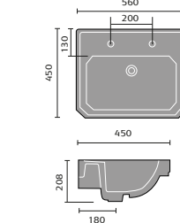
Provence 55cm Semi Recessed Basin
