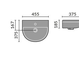
Florence 45cm Cloakroom Basin 1th
