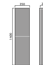
Avior Wall Mounted Tall Cabinet
