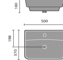
Spacesaver Curved Semi Recessed Basin
