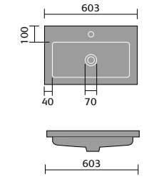
Contemporary 60cm Basin
