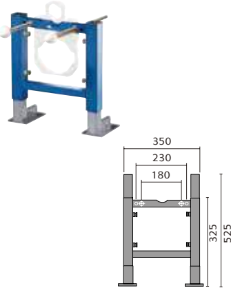
Wall Hung Frame PORIMWF
