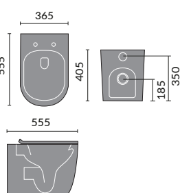
Trivento Back To Wall Toilet
