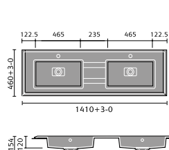
Delphina 1400 Vanity Basin
