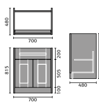
Classic 700 Vanity Floor Standing
