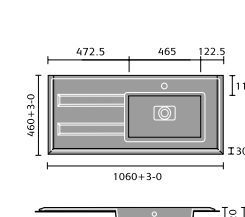
Delphina 1000 Vanity RH Basin
