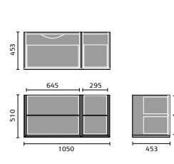
Delphina 1000 Vanity LH
