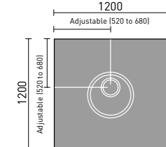
1200mm Smart Deck WRSD12
