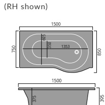
Round Showerbath 1500x850mm LH or RH (RH shown)
