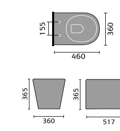
Genoa Back To Wall Toilet
