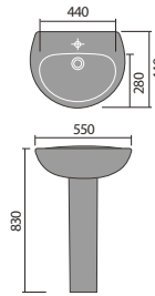
Rimini 55cm Basin 1th and Pedestal
