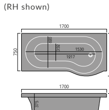
Round Showerbath 1700x850mm LH or RH (RH shown)
