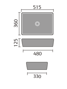
Soft Round Countertop Basin
