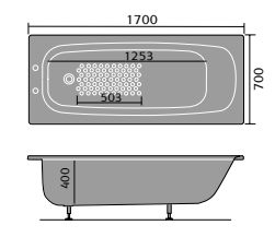
Steel Bath 1700x700mm
