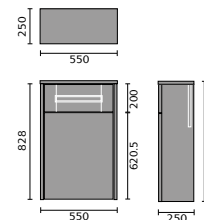
Classic WC Unit
