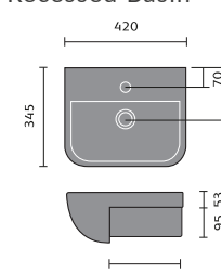
Spacesaver Soft Round Semi Recessed Basin
