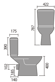
Rimini Open Backed Toilet
