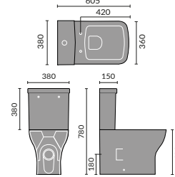
Corsica Open Backed Toilet
