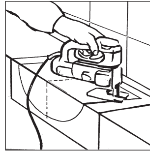
3 Drill hole on the inside of the outer template line.
