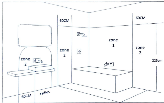
IEE Bathroom Zones Diagram
