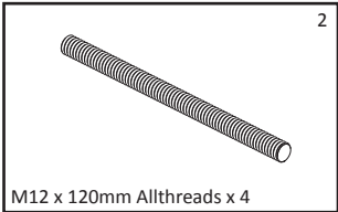
M12 x 120mm Allthreads x 4
