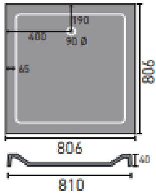
800mm square
