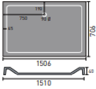
1500 x 700mm rectangular
