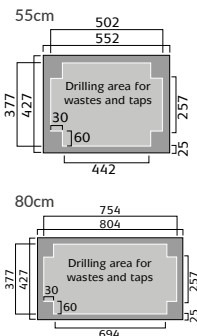
Avior Countertop
