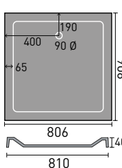
800mm Square
