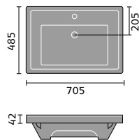
Classic 700 Basin
