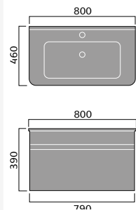
Pavo 800 Vanity
