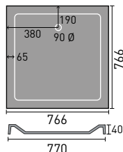
760mm Square
