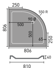
800mm Quad
