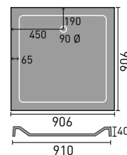
900mm Square
