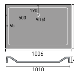
1000x760mm Rectangular
