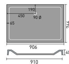
900x760mm Rectangular
