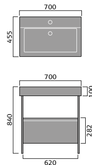
Carina 700 Vanity
