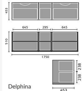
Delphina 1800 Vanity
