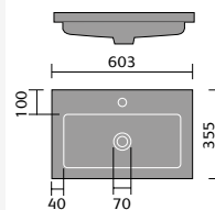
Contemporary Basin
