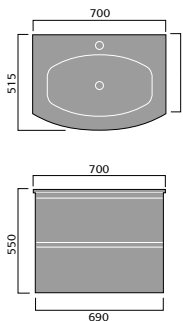
Tauri 700 Vanity
