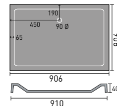
900x800mm Rectangular
