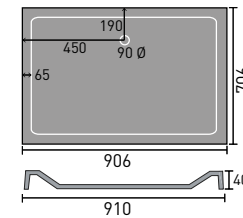
900x700mm Rectangular
