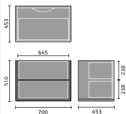
Delphina 700 Vanity
