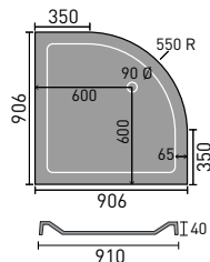
900mm Quad
