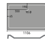
1100x800mm Rectangular
