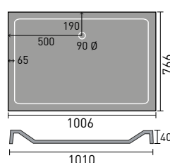
1000x760mm Rectangular
