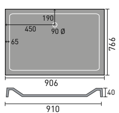
900x760mm Rectangular
