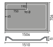
1500x700mm Rectangular
