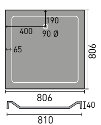
800mm Square
