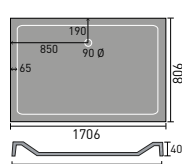
1700x800mm Rectangular
