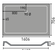
1600x700mm Rectangular
