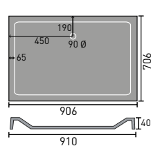
900x700mm Rectangular
