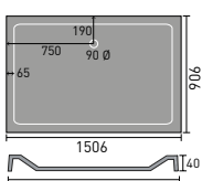
1500x900mm Rectangular
