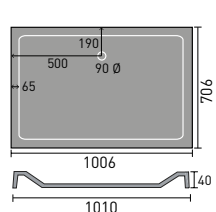
1000x700mm Rectangular
