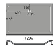
1200x760mm Rectangular
