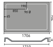
1700x700mm Rectangular
