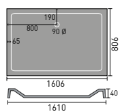
1600x800mm Rectangular
