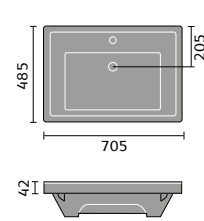
Classic 700 Basin
