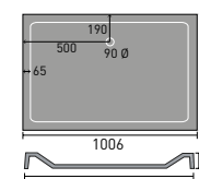
1000x800mm Rectangular
