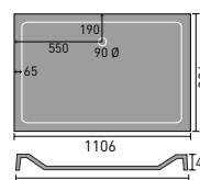
1100x900mm Rectangular
