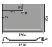
1500x800mm Rectangular
